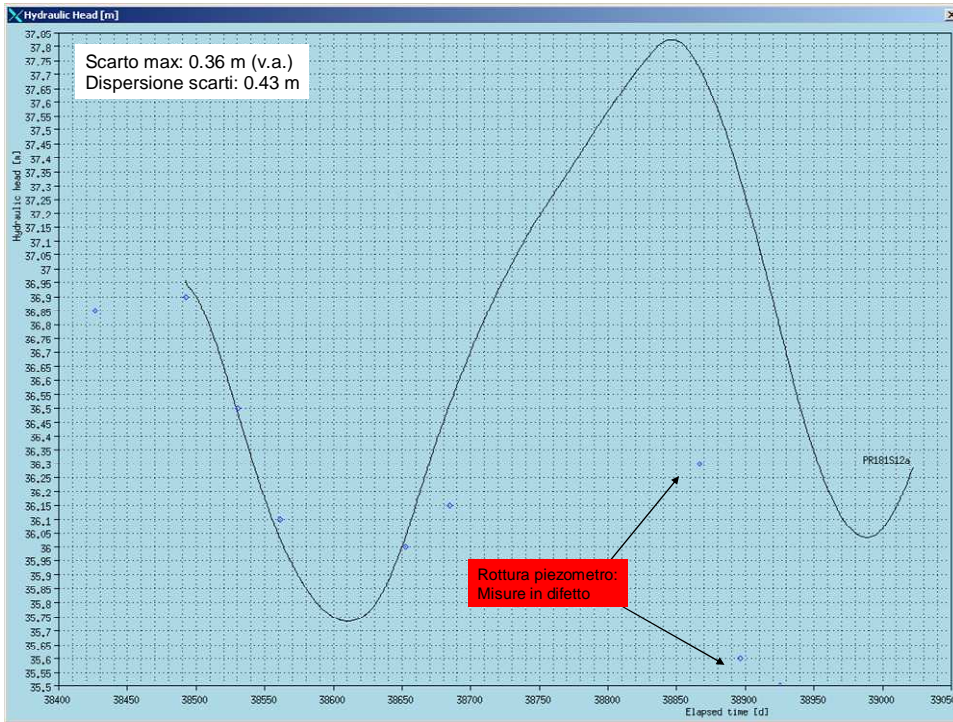
Piezometro PR181S12a
