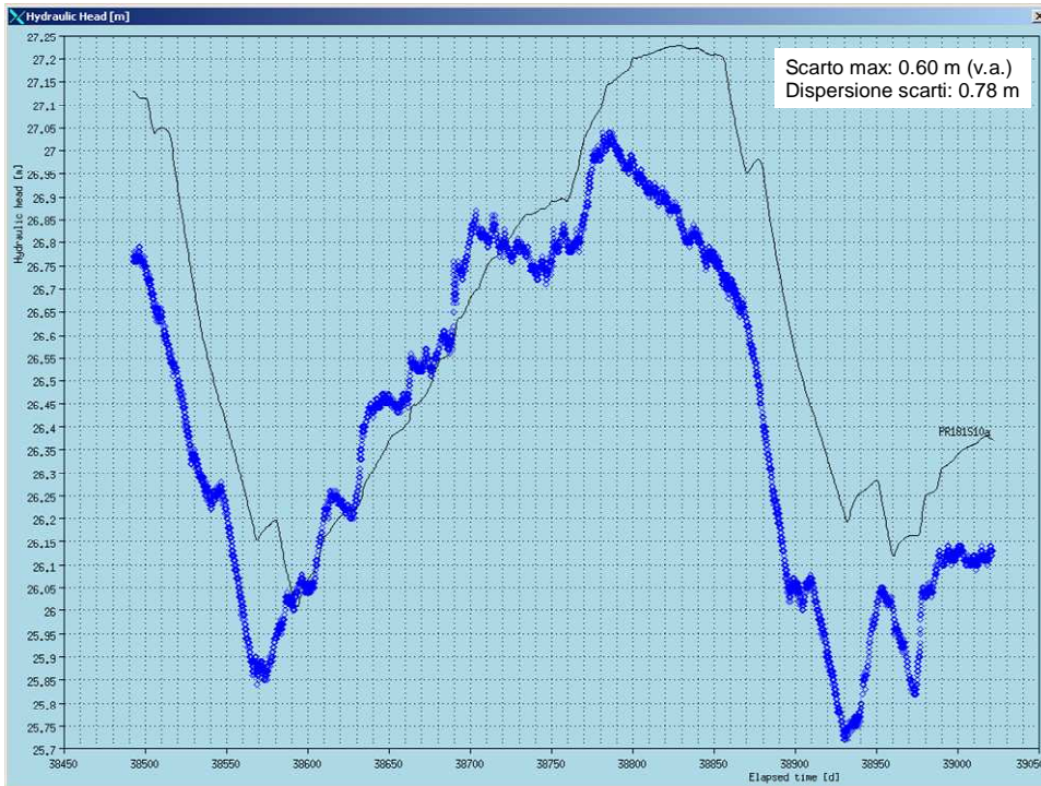
Piezometro PR181S10a
