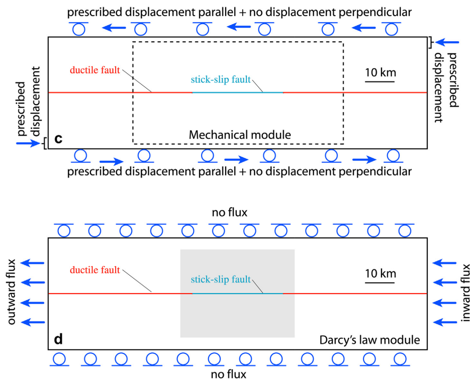
Figure 4. The geometry and boundary conditions for the numerical models of thrust and normal faults (a, b) and strike slip faults (c, d) are shown. In the gray areas, variations of the permeability were allowed, as described in the text. The dashed rectangles indicate the parts of the models shown in Figs. 5–7.
